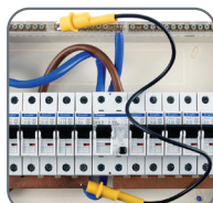
2 long and 2 short leads for 'dead' testing (insulation & R_1 + R_2 testing)
